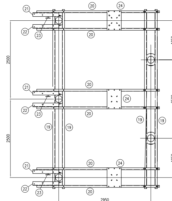
SECTION 3 Scale 1:35
