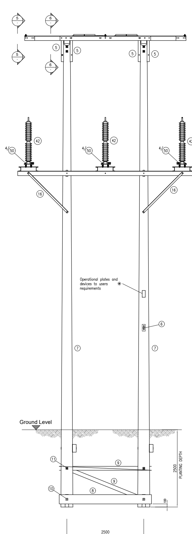
SECTION 1 Scale 1:35
