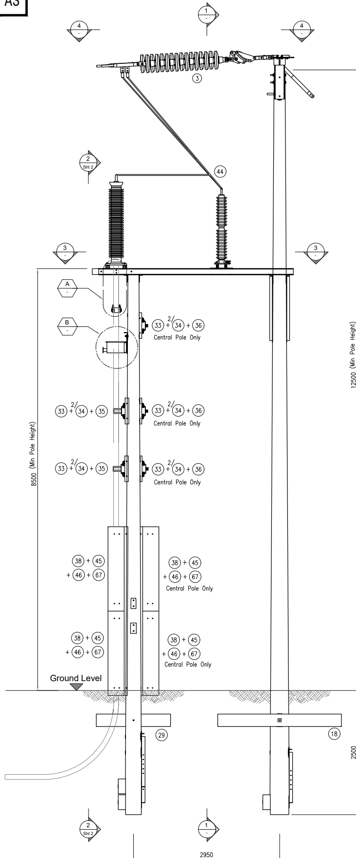
SIDE ELEVATION
